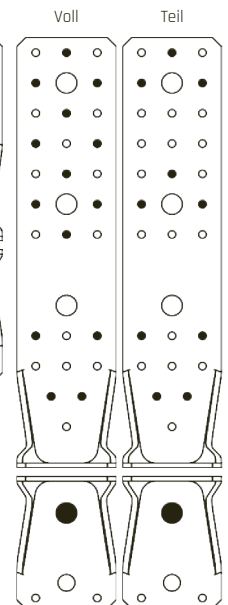
KR Rundloch 285 mm 1102853 / 110285
